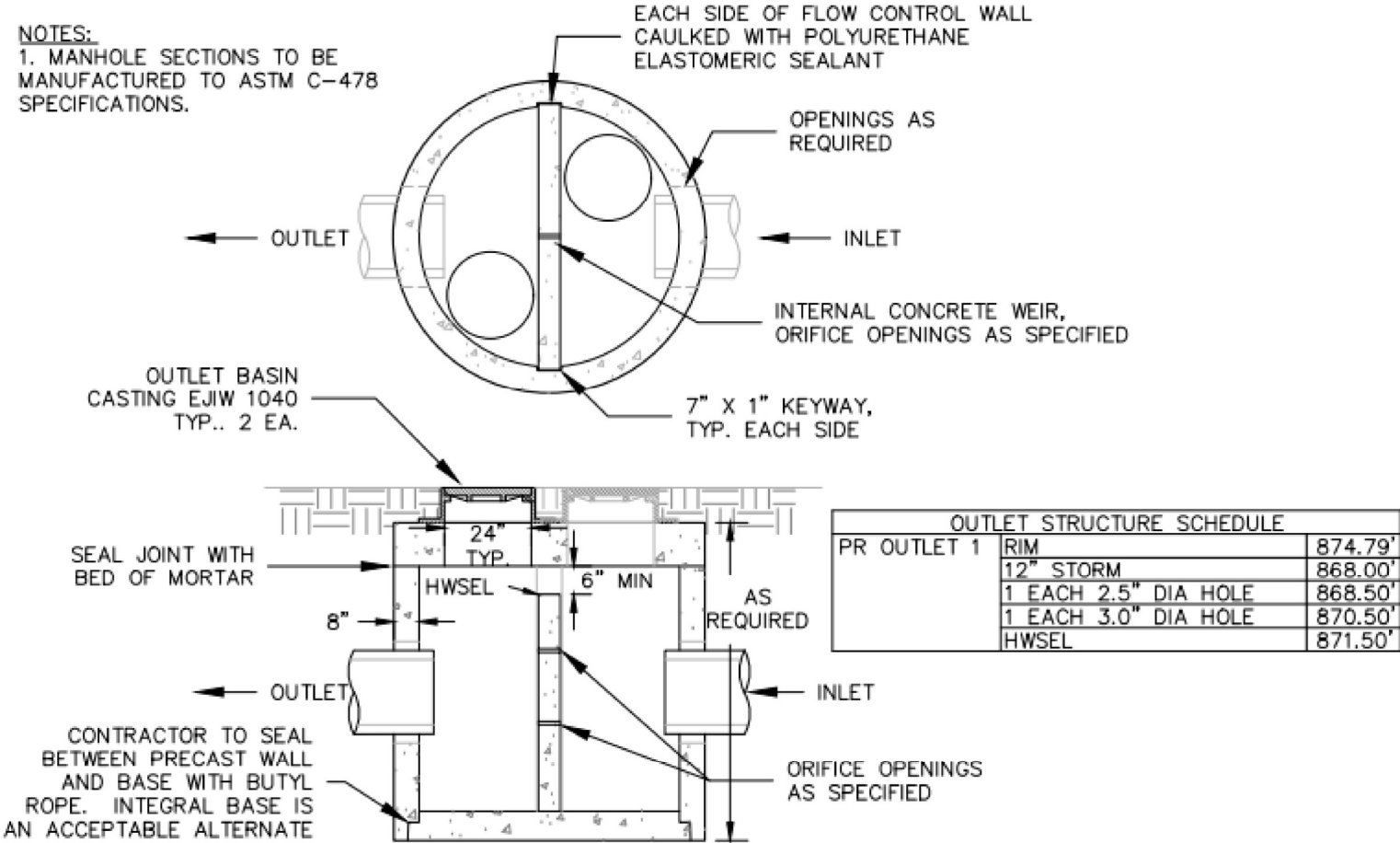
DETENTION POND OUTLET STRUCTURE WITH INTERNAL WEIR
